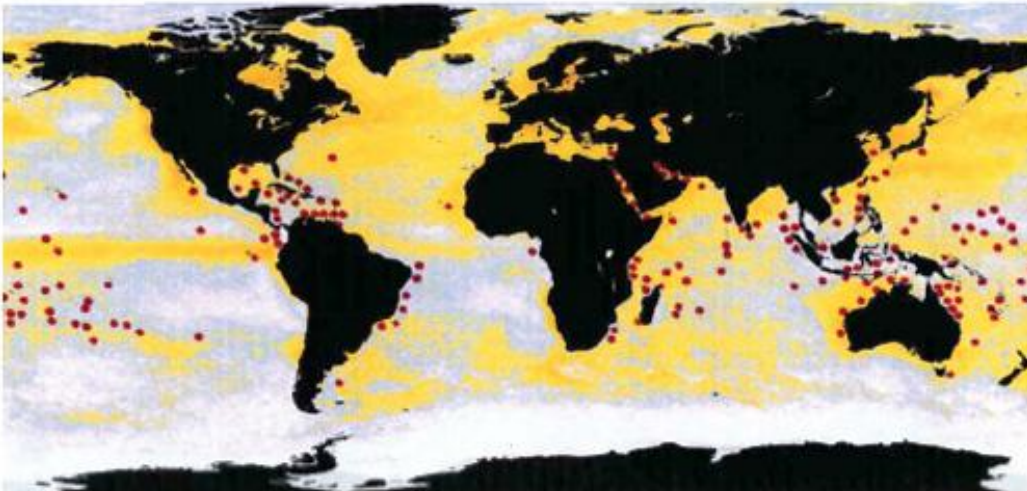
Sea Surface Temperatures and Coral Bleaching
